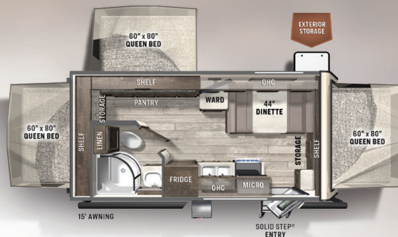
183 EXPANDABLE U/VW: 4137 HITCH: 448 AXLE: 3651 LENGTH: 21'2" OPEN LENGTH: 25'7" ROO CCC: 1591 WIDTH: 8' HEIGHT: 10'6" FRESH: 54 gal GRAY: 30gal BLACK: 30gal
