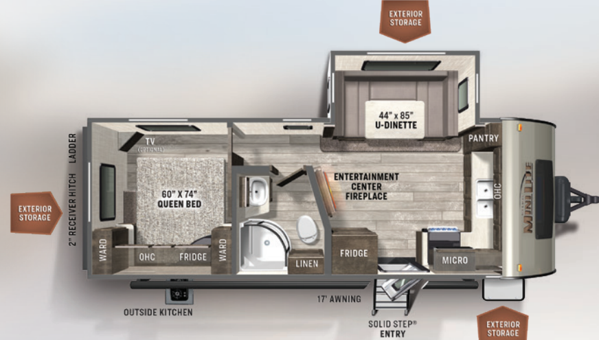
2506S FRONT KITCHEN UVW: 5281 HITCH: 644 AXLE: 4510 CCC: 1523 LENGTH: 25'11" MINI LITE WIDTH: 8' HEIGHT: 10'11" FRESH: 54 gal GRAY: 60 gal BLACK: 30 gal
