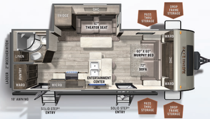
2514S MURPHY BED UVW: 5879 HITCH: 585 AXLE: 5235 CCC: 1706 LENGTH: 25'10" MINI LITE WIDTH: 8' HEIGHT: 10'11" FRESH: 54 gal GRAY: 30 gal BLACK: 30 gal
